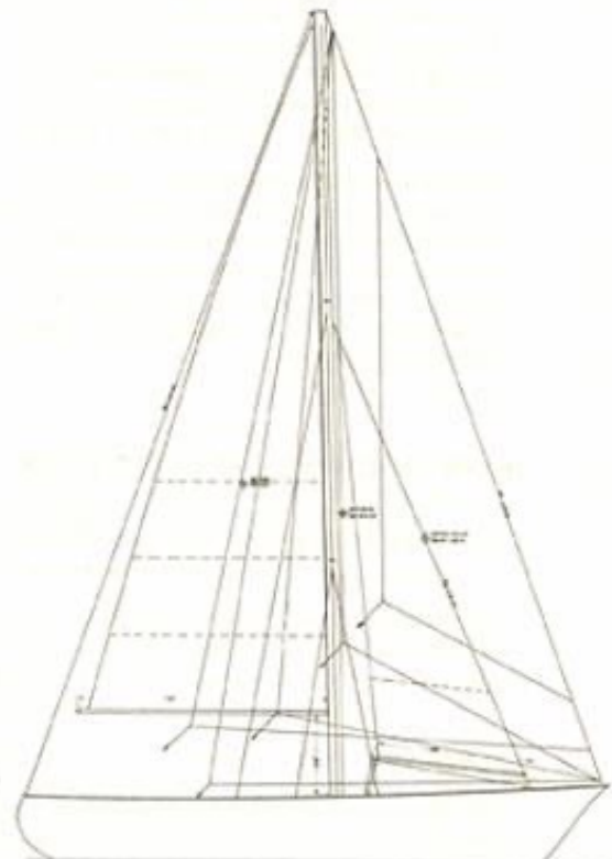
TALL RIG CUTTER
